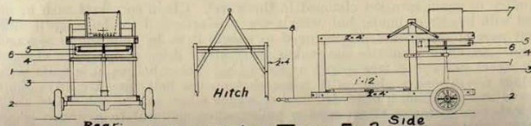
Auto-Trailer Type. Fig. 2
